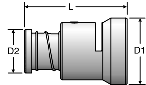
Fig. R112 — Captive O-Ring Assembly Tool dimensions
